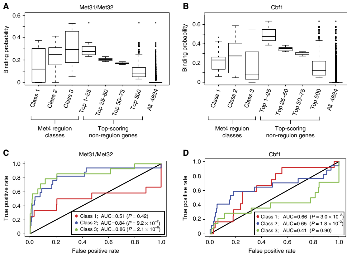
Figure 3 Specificity of Met32- and Cbf1-specific binding models for Met4 regulon genes. (A, B) Probability distribution for Met32 and Cbf1 binding to gene promoters from different gene sets. Met4 regulon genes are grouped according to Met4 regulon class designation of Lee et al (2010) and non-regulon genes are grouped into the top-scoring gene sets of 25 genes (3 sets) and top-scoring 500 genes (1 set). (C, D) ROC curve analysis for the prediction of each regulon gene class using the 500 top-scoring background (i.e., non-regulon) genes as false positives. Genes are scored and ranked according to the Met32-specific and Cbf1-specific binding probabilities calculated for each gene promoter (Materials and methods). Wilcoxon–Mann–Whitney U -test was applied to each regulon gene set to calculate significance of the AUC values.
